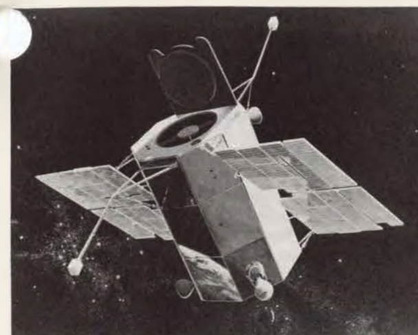
ORBITAL ASTRONOMICAL OBSERVATORY
