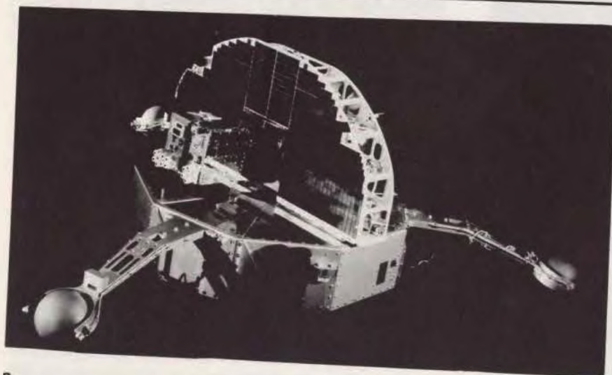
1. APOLLO TELESCOPE MOUNT 2. ORBITING SOLAR OBSERVATORY 3. RADIO ASTRONOMY EXPLORER
