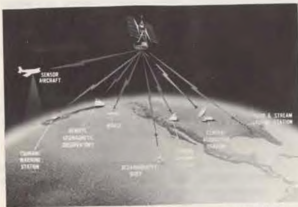
EARTH RESOURCE SURVEY DATA WHICH CAN BE COLLECTED BY SATELLITE
