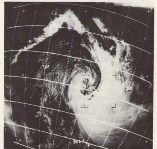
EXTRATROPICAL STORM VIEWED BY ESSA-III
